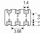
Underside View
