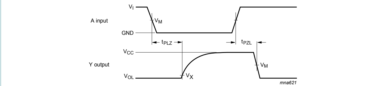
Figure 8. The data input (A) to output (Y) propagation delays
