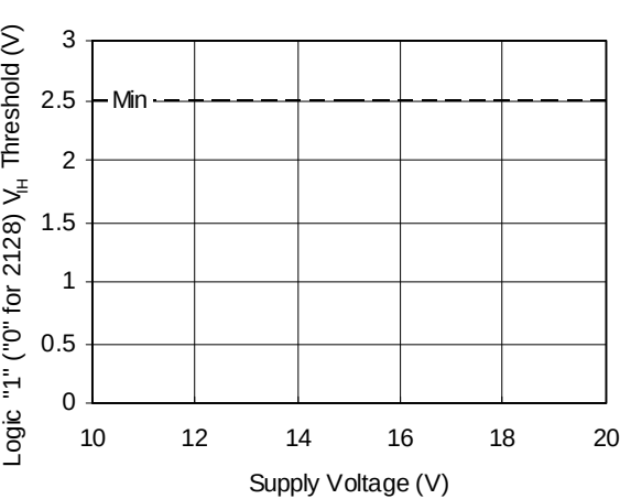
Figure 13B. Logic "1" ("0" for 2128) V_{IH} Threshold vs. Voltage
