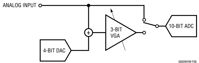
Figure 8. Analog Input Chain
