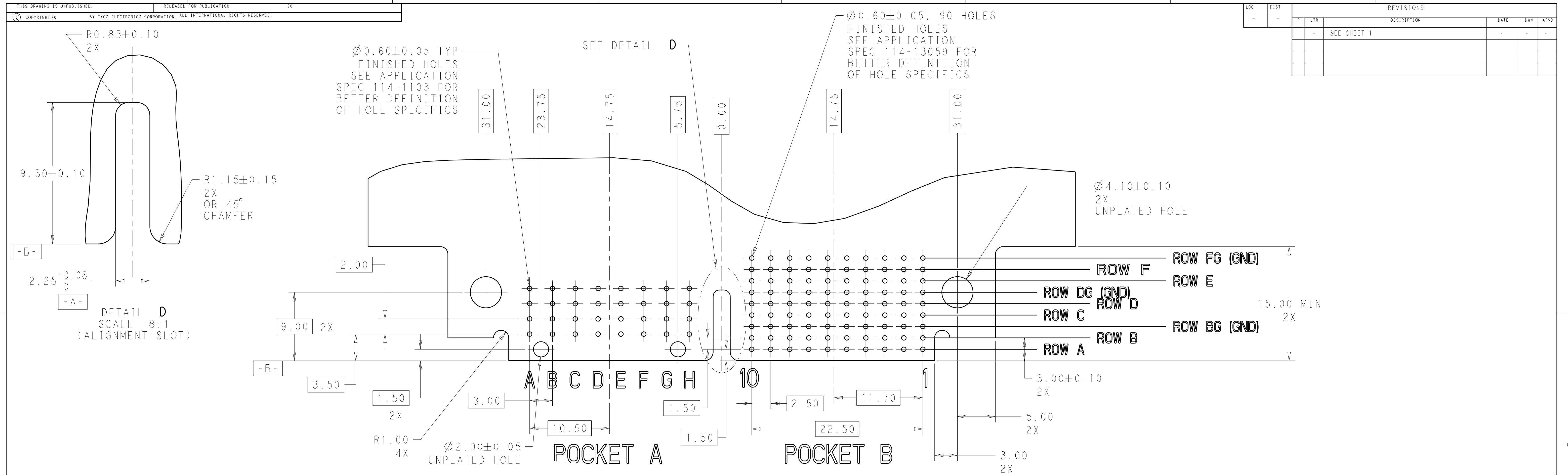
RECOMMENDED PRINTED CIRCUIT BOARD LAYOUT AS VIEWED FROM TOP OF PRINTED CIRCUIT BOARD
