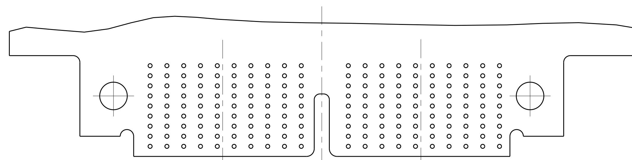
2033993-3 PCB SCALE 3:1
