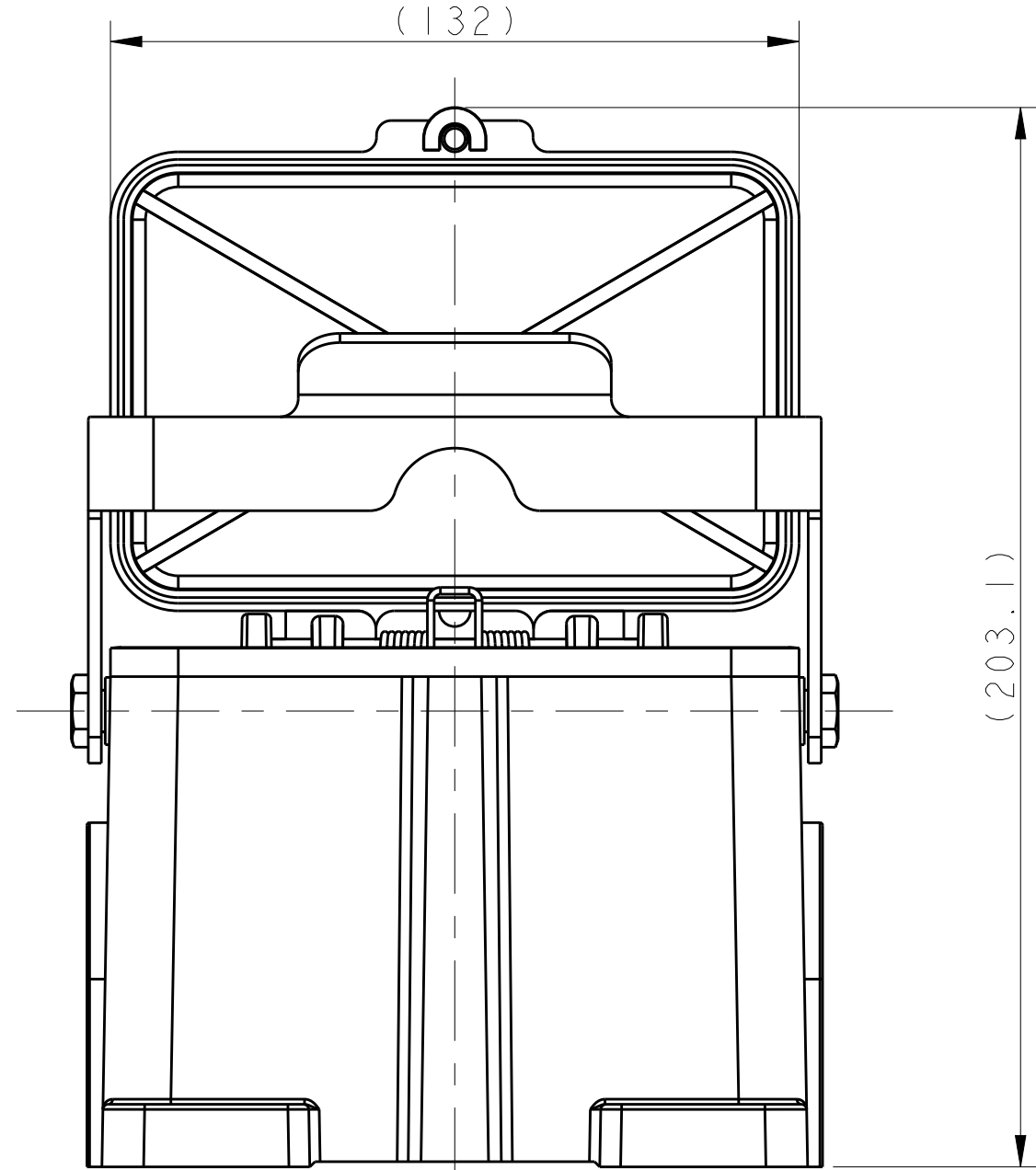
TYPE 2: H48 HOUSING, SURFACE MOUNTED, STAINLESS STEEL SINGLE LOCKING WITH PLASTIC PROTECTION COVER, OTHER SPEC REFER TO TYPE 1
