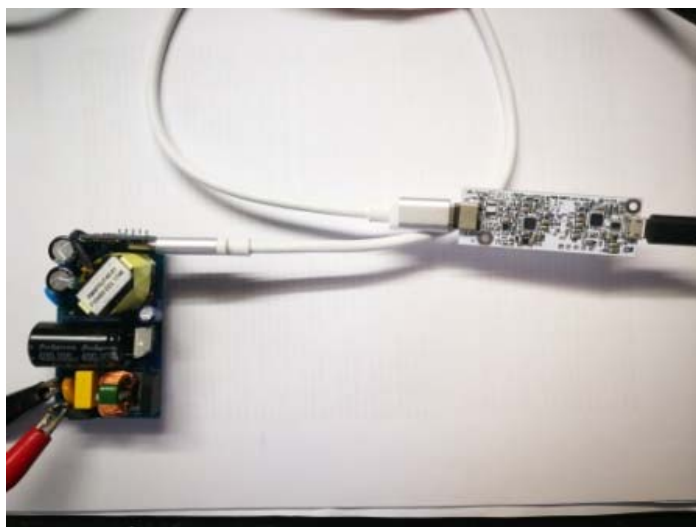
Figure 7: EVKT-MPX2001-45-PD Hardware Setup
