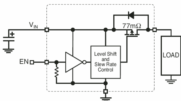
½ MIC94066, 68 Load Switch Application
