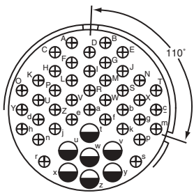
110° Rotation of 36-7 36-17
