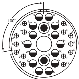
100° Rotation of 36-9 36-18
