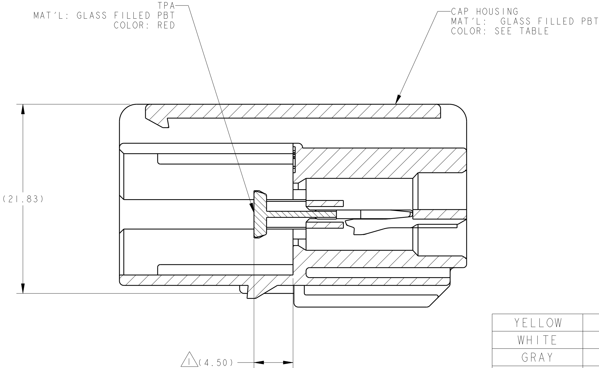
SECTION Z-Z
