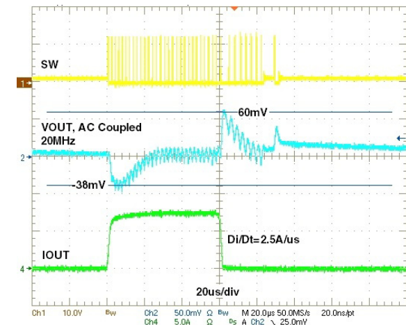
Figure 18: Load step, DCM/CCM, 0A-7.5A-0A
