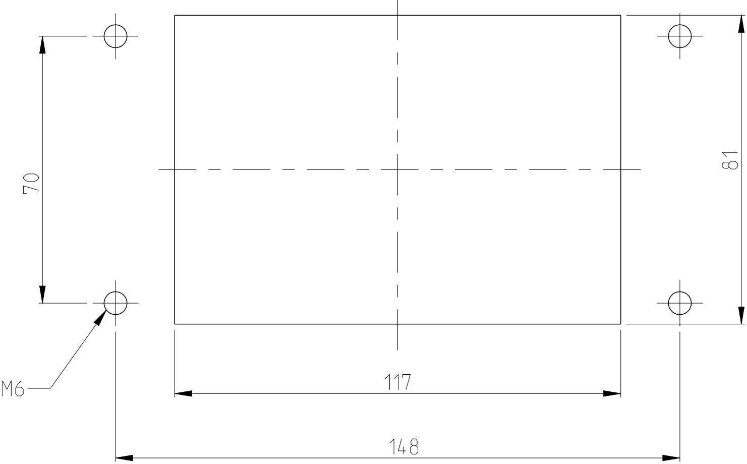
PANEL CUT-OUT
