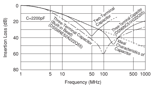
Comparison of Insertion Loss Characteristics
