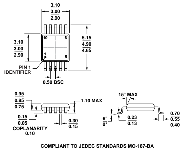
Figure 44. 10-Lead Mini Small Outline Package [MSOP] (RM-10)
