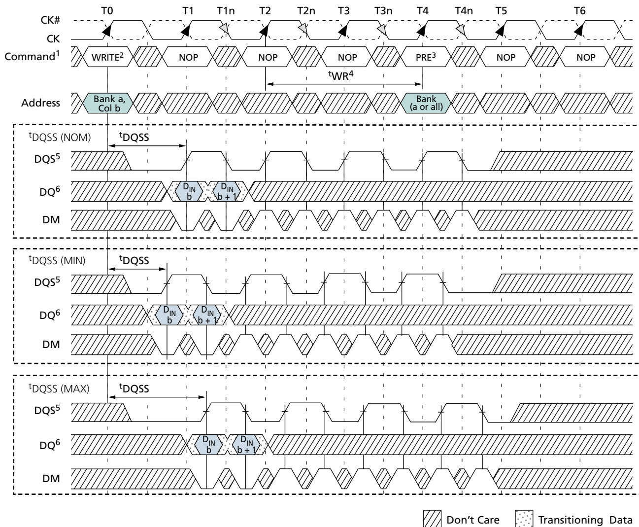
Figure 43: WRITE-to-PRECHARGE – Interrupting
