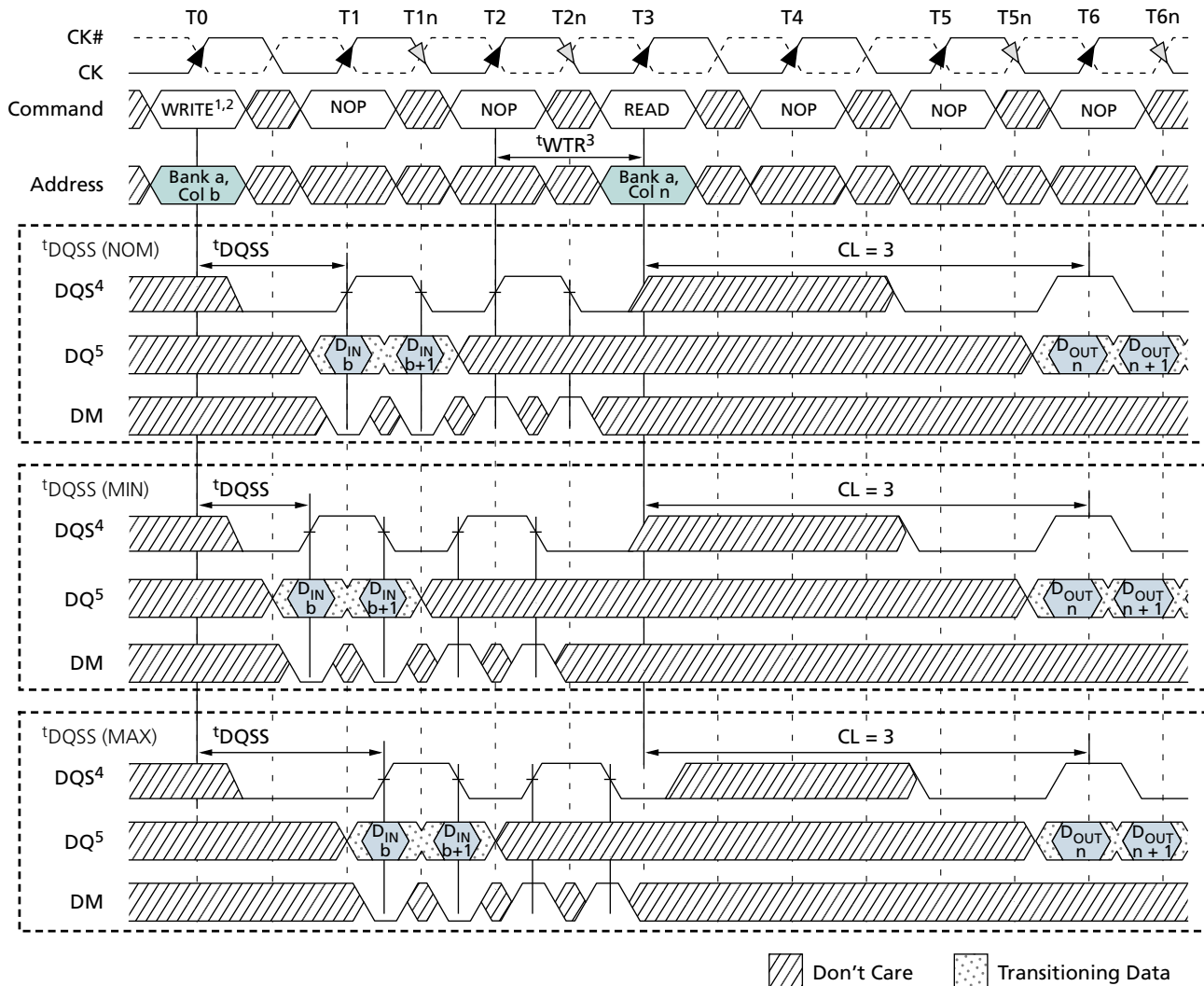
Figure 40: WRITE-to-READ – Interrupting
