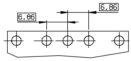
LAYOUT DIMENSIONS (after plating) CONNECTOR SIDE VIEW
