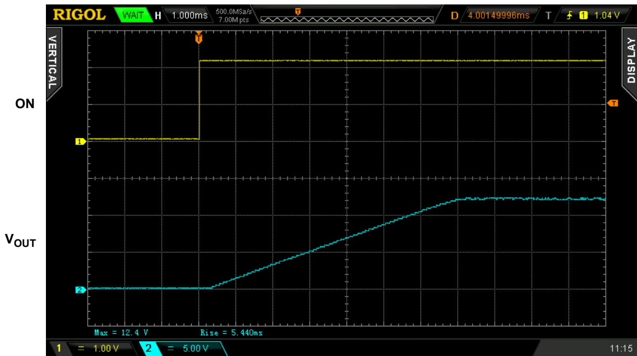
Figure 2. Typical Turn ON operation waveform for V_{IN} = 12\text{ V} , C_{SLEW} = 18\text{ nF} , C_{LOAD} = 10\text{ μF} , R_{LOAD} = 100\text{ Ω}
