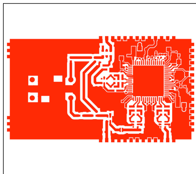
SC1905-DB2400—PCB Layout—Top
