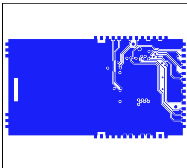
SC1905-DB3400—PCB Layout—Bottom
