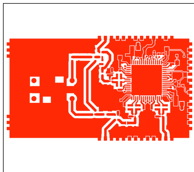
SC1905-DB3400—PCB Layout—Top
