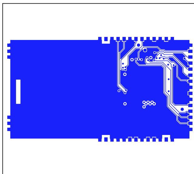
SC1905-DB1900—PCB Layout—Bottom
