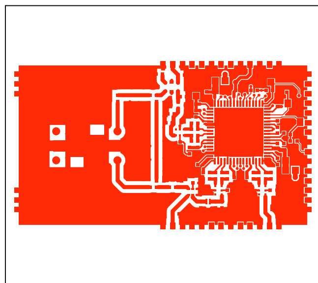
SC1905-DB1900—PCB Layout—Top
