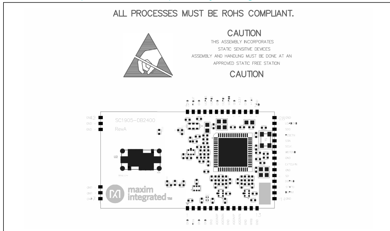
SC1905-DB2400—Assembly Drawing
