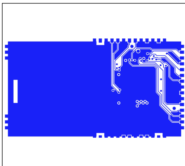
SC1905-DB2400—PCB Layout—Bottom
