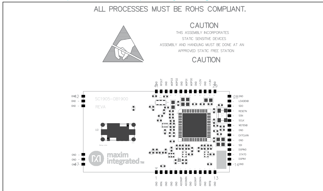
SC1905-DB1900—Assembly Drawing
