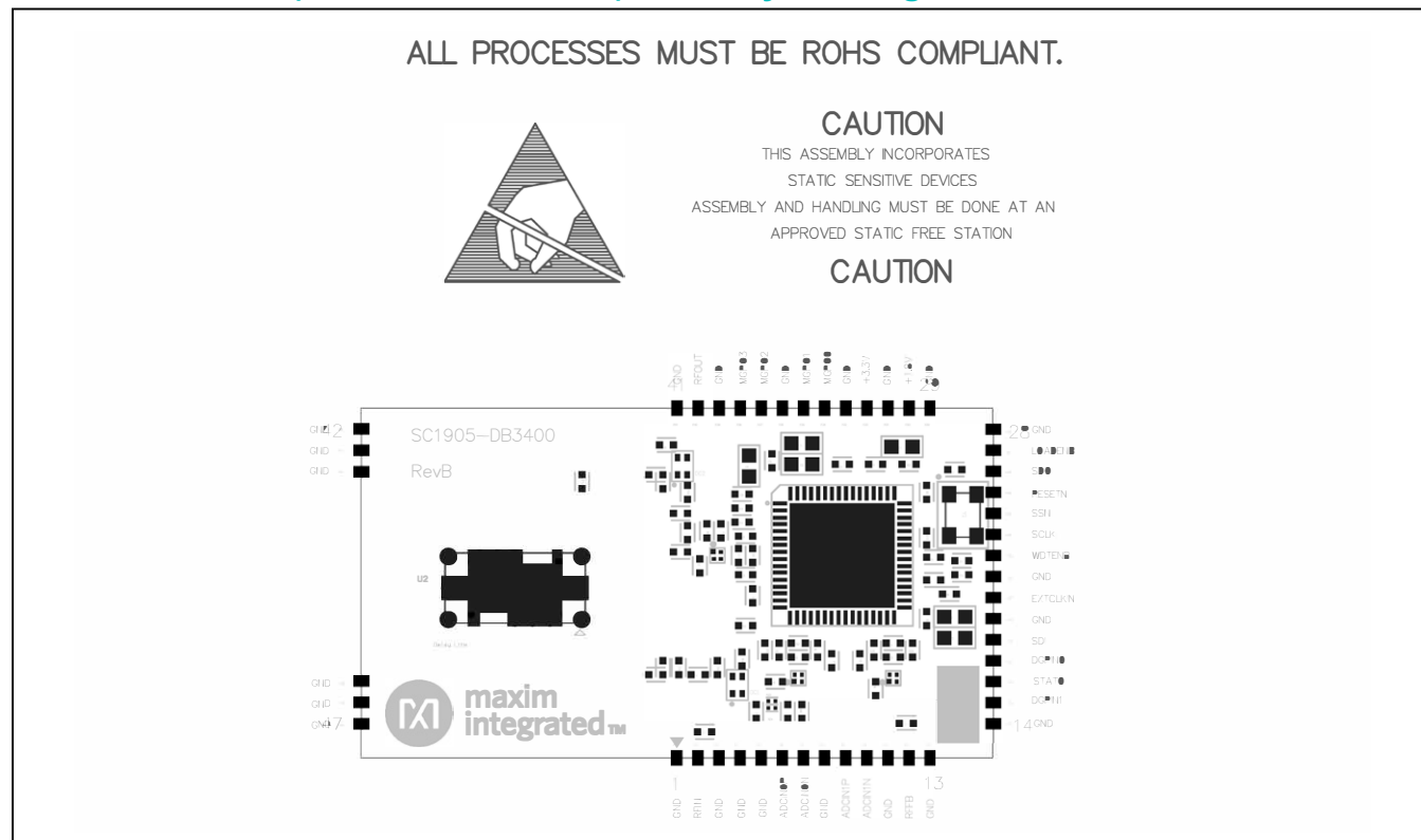
SC1905-DB3400—Assembly Drawing
