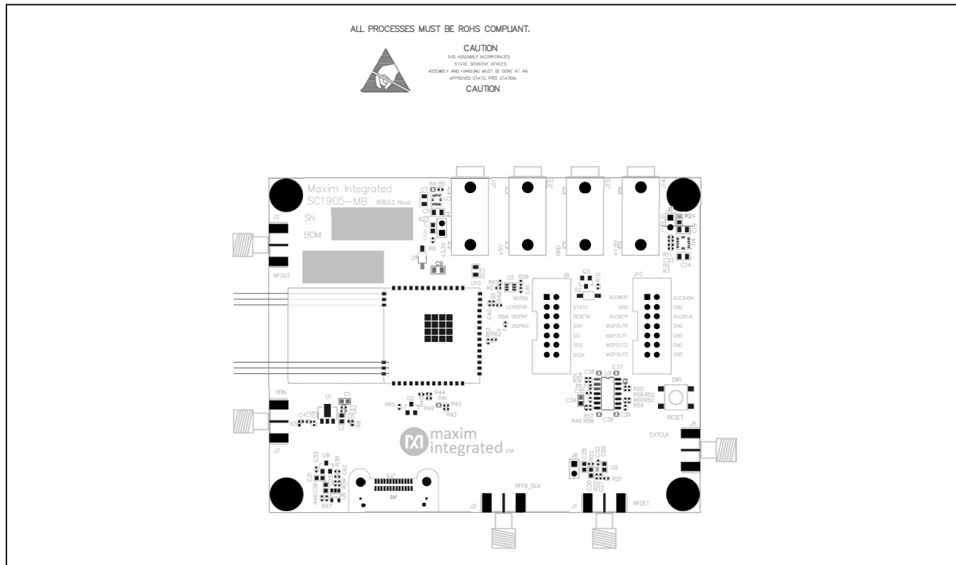
SC1905-MB—Assembly Drawing
