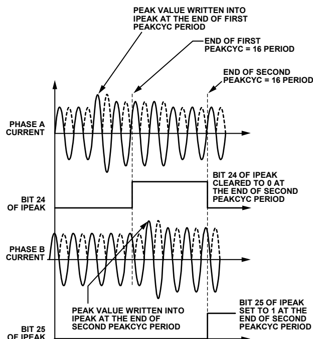
Figure 61. Peak Level Detection
