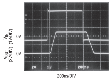
Output-Overdrive Recovery
