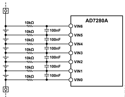
Figure 33. External Series Resistance and Shunt Capacitance
