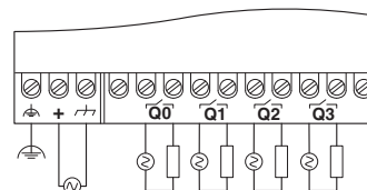
Connection diagram
