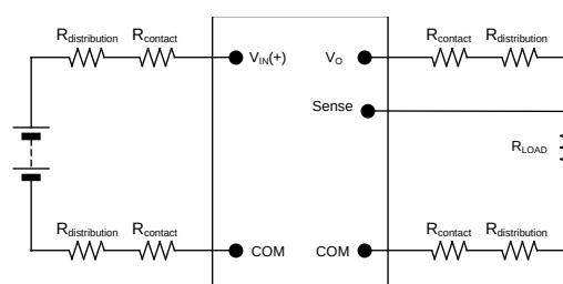
Figure 31. Remote sense circuit configuration.
