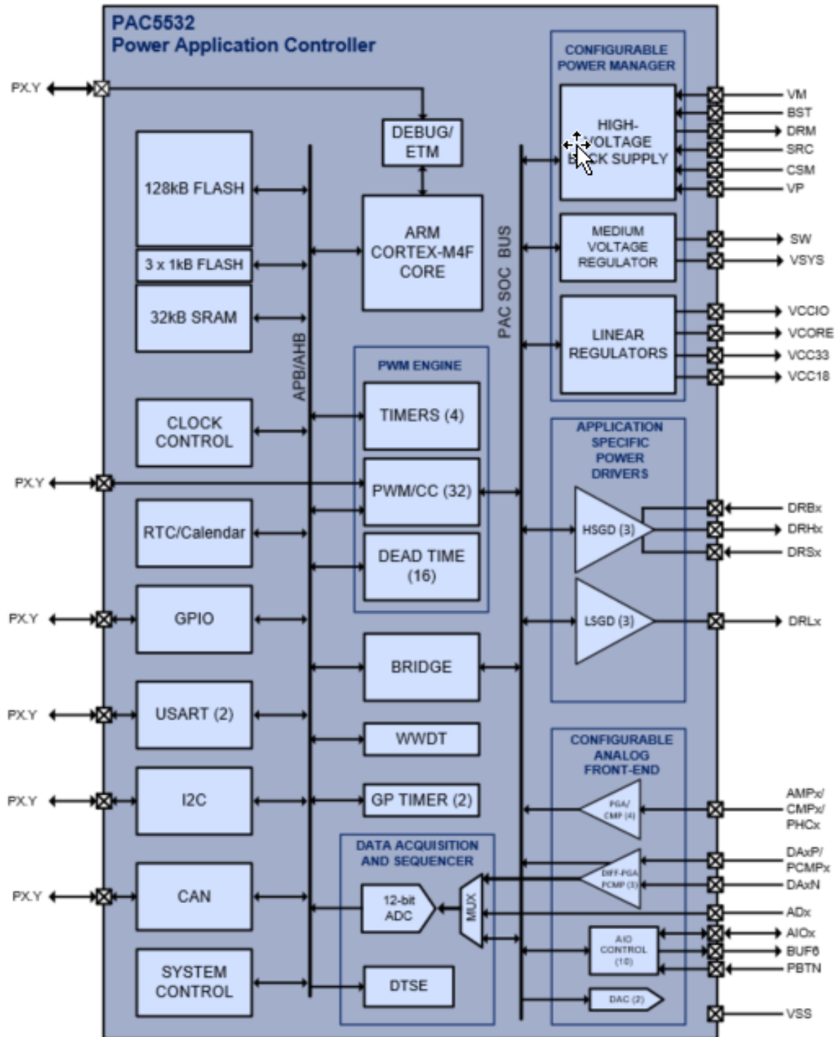
Figure 7-1 Architectural Block Diagram
