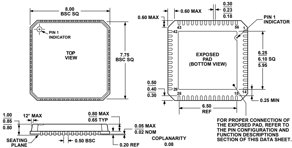
COMPLIANT TO JEDEC STANDARDS MO-220-VLLD-2 Figure 44. 56-Lead Lead Frame Chip Scale Package [LFCSP_VQ] 8 mm × 8 mm Body, Very Thin Quad (CP-56-1) Dimensions shown in millimeters
