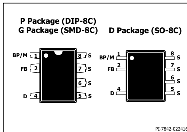
Figure 4. Pin Configuration.
