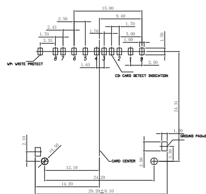
RECOMMENDED PCB LAYOUT (ALL TOLERANCE ARE ±0.05)
