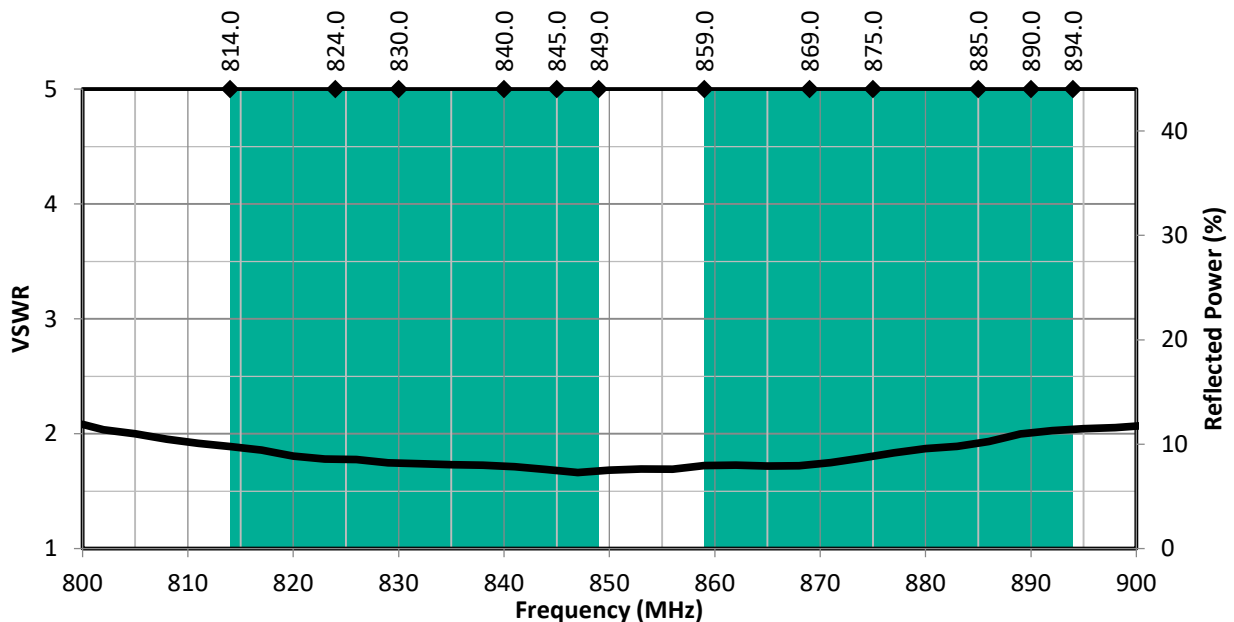
Figure 1. CW LTE Band 5 Antenna VSWR with Band 5 Uplink/Downlink Highlights
