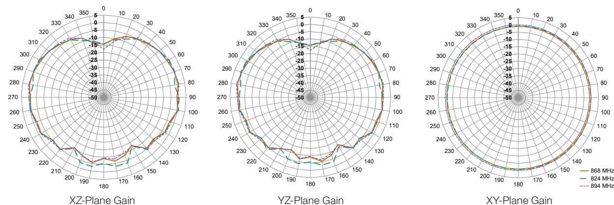
Figure 8. Radiation Patterns for CW LTE Band 5 Antenna
