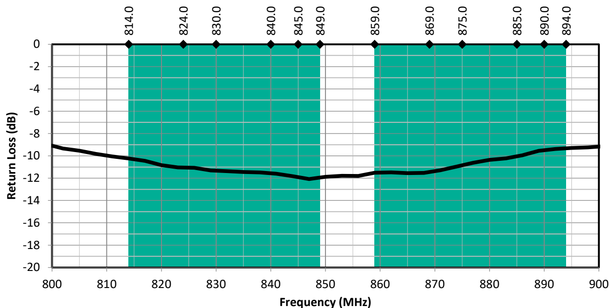
Figure2. CW LTE Band 5 Antenna Return Loss with Band 5 Uplink/Downlink Highlights
