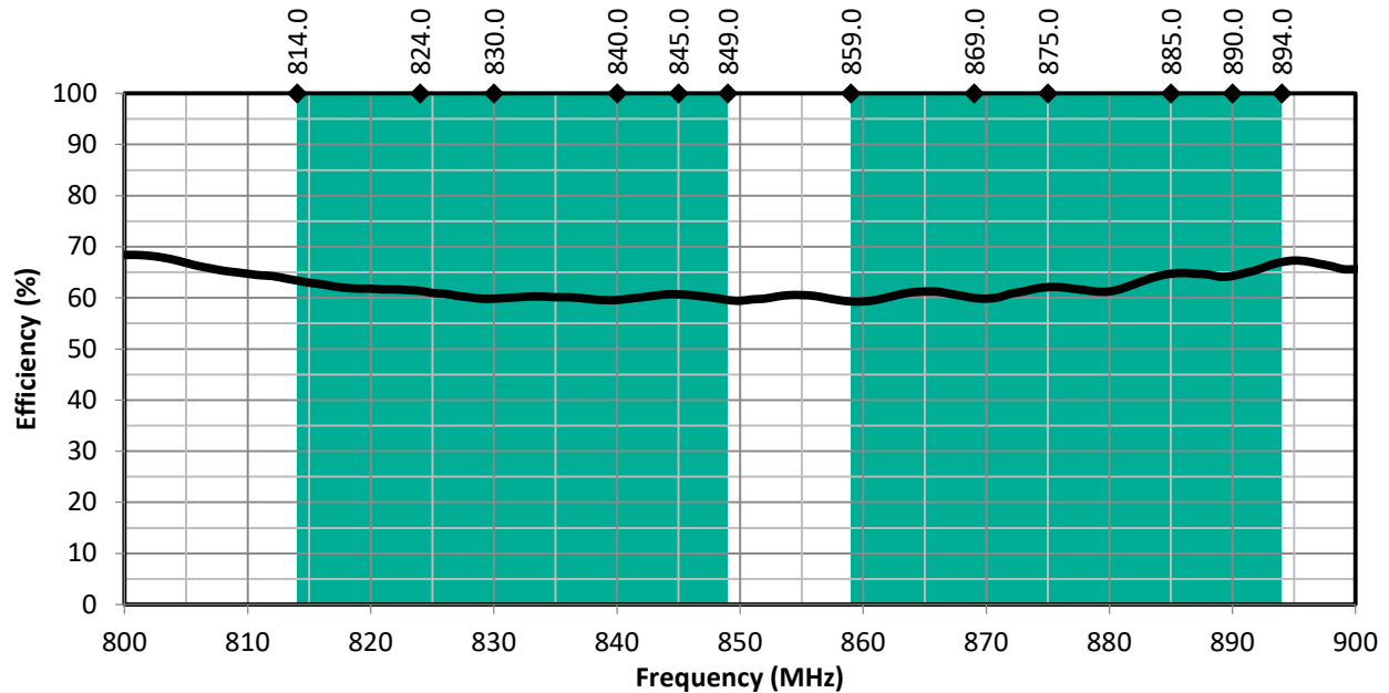
Figure 5. CW LTE Band 5 Antenna Radiation Efficiency with Band 5 Uplink/Downlink Highlights
