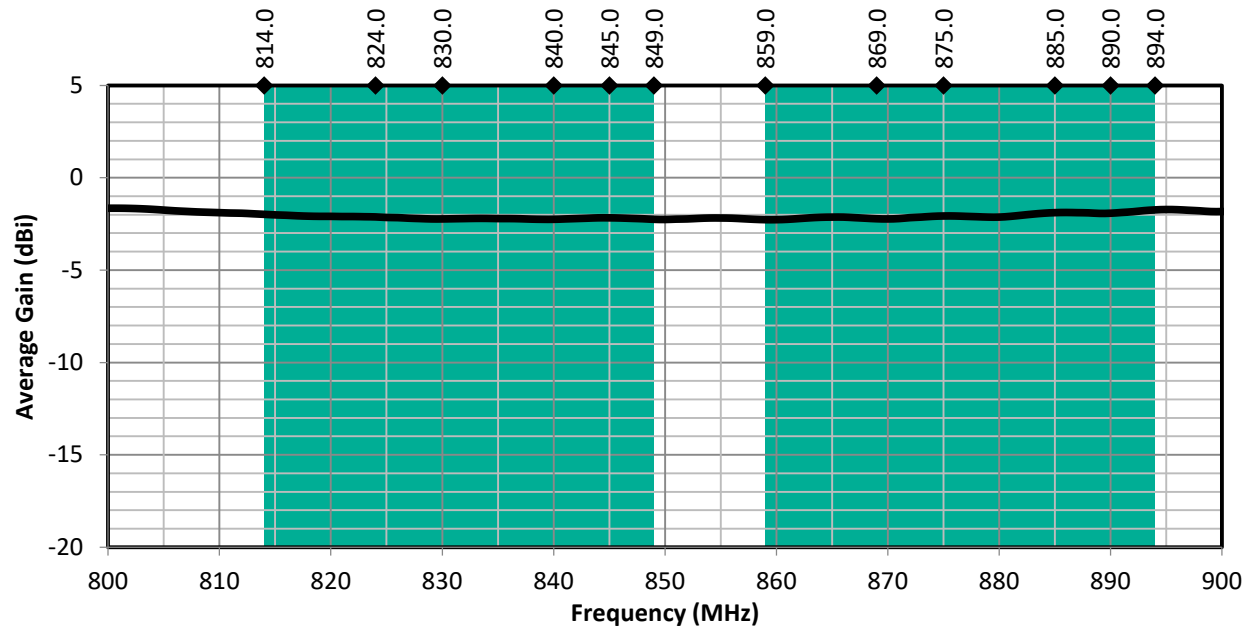
Figure 4. CW LTE Band 5 Antenna Average Gain with Band 5 Uplink/Downlink Highlights
