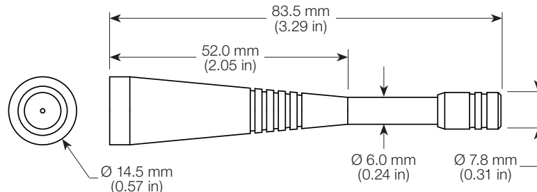
Figure 6. CW LTE Band 5 Antenna Dimensions
