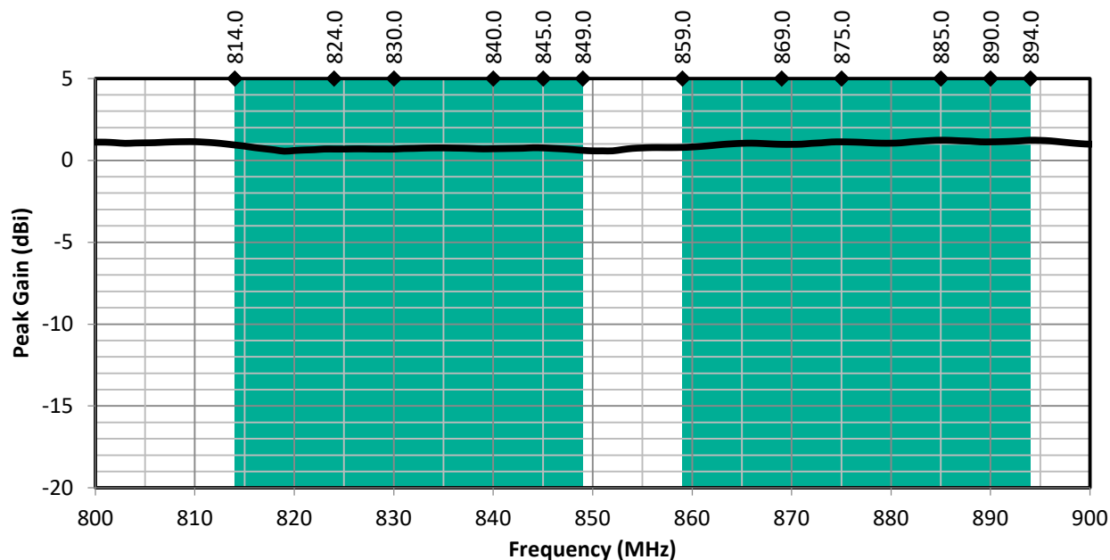
Figure3. CW LTE Band 5 Antenna Peak Gain with Band 5 Uplink/Downlink Highlights
