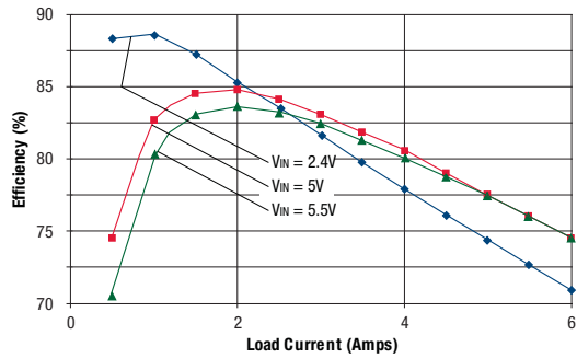
Efficiency vs. Line Voltage and Load Current @ +25°C ( V_{OUT} = 0.6V )
