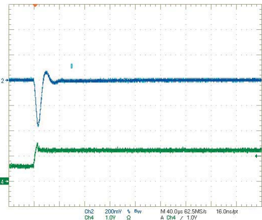
Step Load Transient Response ( V_{IN} = 5V , V_{OUT} = 1.0V , I_{OUT} = 3A to 6A) Trace 2=Vout, 200 mV/div. Trace 4=Iout, 5A/div.
