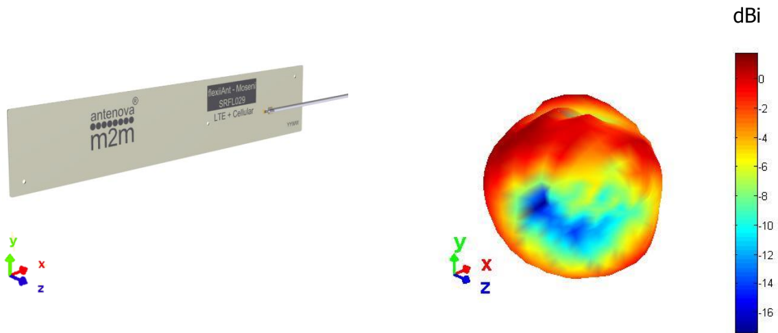
3D pattern at 745 MHz Drag to rotate pattern and PCB by using Adobe Reader (Click to Activate)
