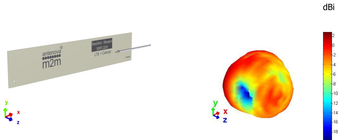
3D pattern at 890 MHz Drag to rotate pattern and PCB by using Adobe Reader (Click to Activate)
