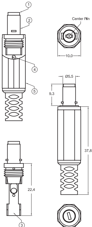
KLDX-PA-0202-x-LT Assembly type, Locking
