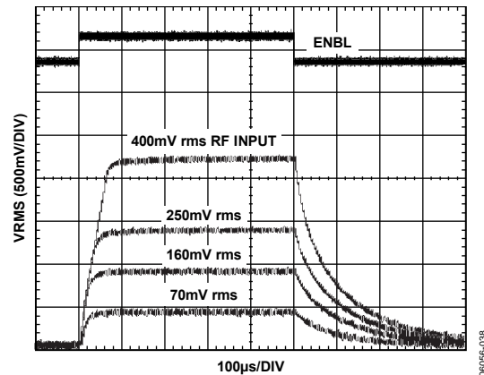
Figure 38. Output Response to Enable Gating at Various RF Input Levels, Supply = 3 V, Frequency = 900 MHz, C_{FLTR} = \text{Open} , C_{OUT} = 0.1 μF, R_{OUT} = 1 kΩ
