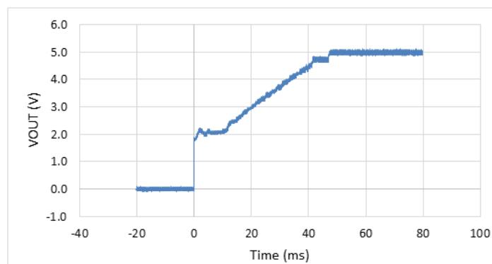
Figure 4.22. 24 V-5 V VOUT Startup vs. Time, 400 mA Load Current
