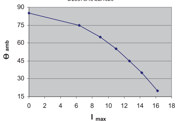
Max. allowable ambient Temp. at specific current (rms) B25673A5102A020
