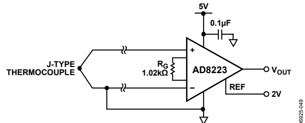
Figure 42. Amplifying Bipolar Signals with Low Common-Mode Voltage
