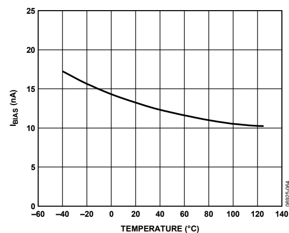
Figure 7. I_{BIAS} vs. Temperature
