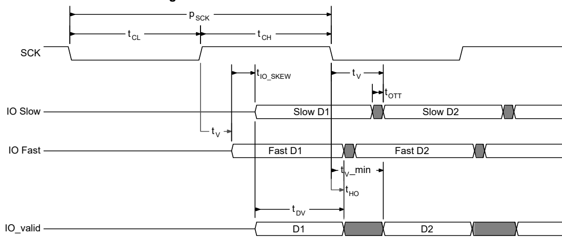
Figure 149. SPI DDR Data Valid Window
