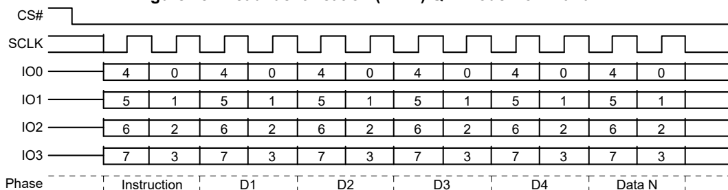
Figure 28. Read Identification (RDID) QPI Mode Command
