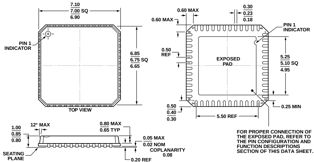
Figure 45. 48-Lead Lead Frame Chip Scale Package [LFCSP_VQ] 7 x 7 mm Body, Very Thin Quad (CP-48-1) Dimensions shown in millimeters
