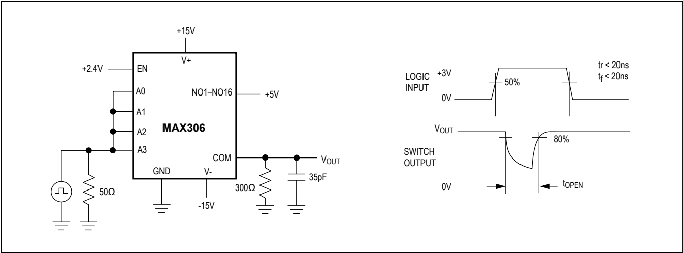
Figure 4. Break-Before-Make Interval
