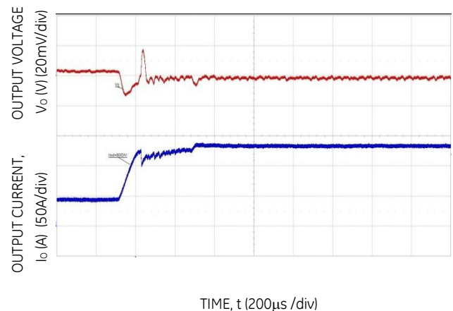
Figure 4. Transient Response to Dynamic Load Change from 25% to 75% at 12V in , C_o = 12 \times 47\mu\text{F} + 10 \times 1000\mu\text{F} , R_{TUNE} = 3.01\text{k}\Omega .
