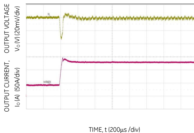
Figure 28. Transient Response to Dynamic Load Change from 25% to 75% at 12Vin, C_O = 12 \times 47\mu\text{F} + 10 \times 1000\mu\text{F} , R_{TUNE} = 3.01\text{k}\Omega .
