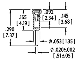
SOLDER TAIL
