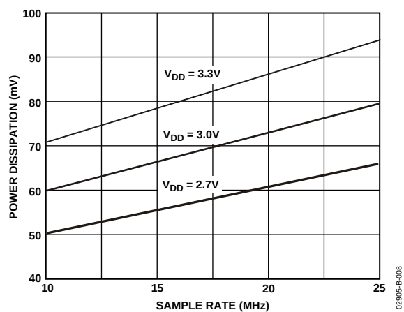
Figure 7. AD9943/AD9944 Power vs. Sample Rate
