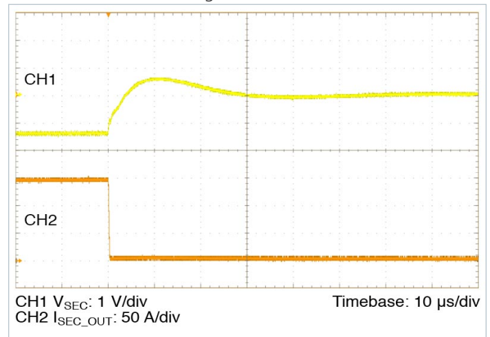
Figure 13 — 160 A – 0 A transient response: C_{IN} = 270 \mu F , no external C_{SEC\_OUT\_EXT}
