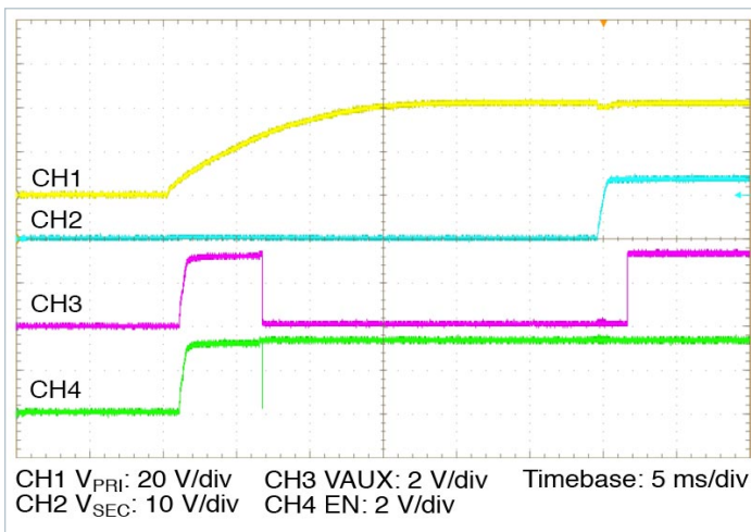
Figure 14 — Start up from application of V_{PRI\_DC} = 42 V , 20% I_{OUT} , 100% C_{SEC\_OUT\_EXT}
