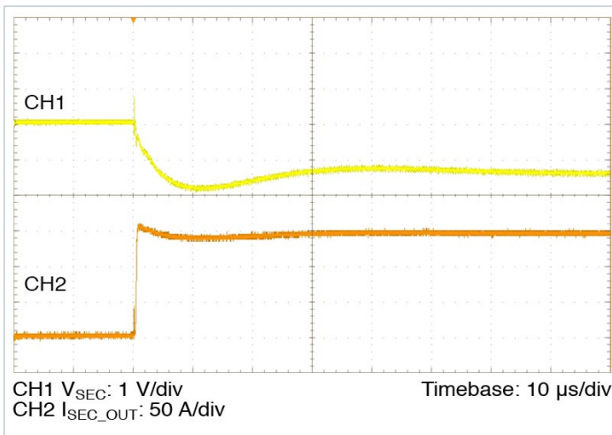
Figure 12 — 0 A– 160 A transient response: C_{PRI\_OUT\_EXT} = 270 \mu F , no external C_{SEC\_OUT\_EXT}
