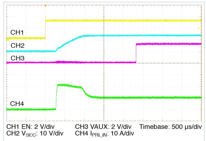
Figure 15 — Start up from application of EN with pre-applied V_{PRI\_DC} = 42 V , 20% I_{SEC\_DG} , 100% C_{SEC\_OUT\_EXT}
