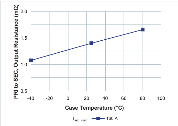
Figure 9 — R_{OUT} vs. temperature; Nominal V_{PRI\_DC} I_{SEC\_DC} = 160\text{ A} at T_{CASE} = 80^{\circ}C
