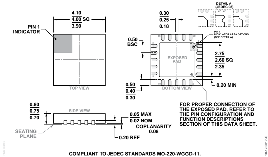
Figure 56. 20-Lead Lead Frame Chip Scale Package [LFCSP] 4 mm × 4 mm Body and 0.75 mm Package Height (CP-20-8) Dimensions shown in millimeters
