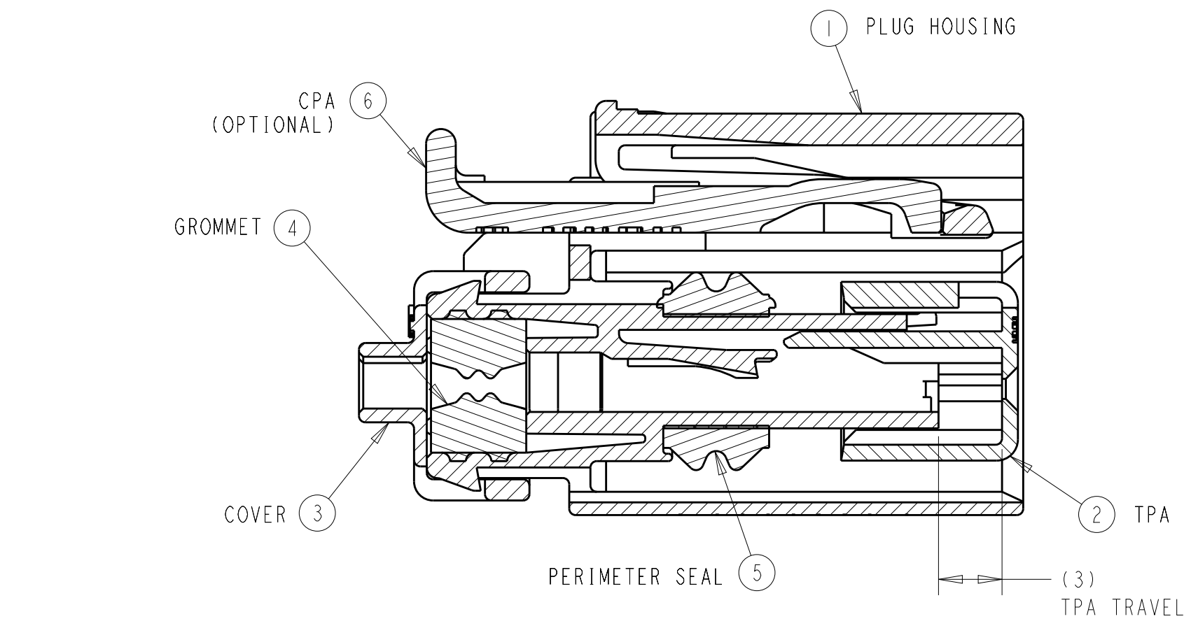
SECTION A-A SHOWN WITH TPA AND CPA (OPTIONAL) IN THEIR PRE-LOADED POSITION (DELIVERY CONDITION)
