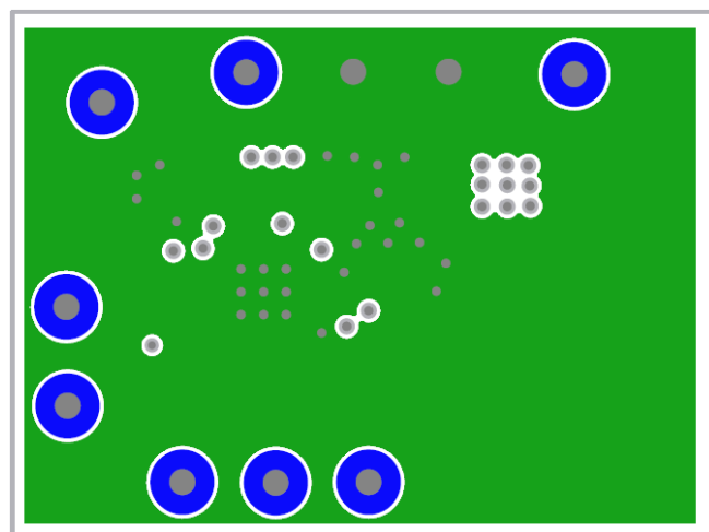
FIGURE 15. 2 nd LAYER
