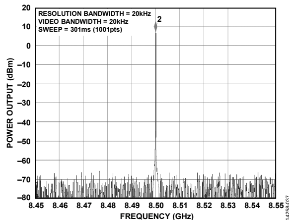
Figure 33. Results of the ADL5721 with an Input of 8.5 GHz at –15 dBm, BAND = 1.8 V
