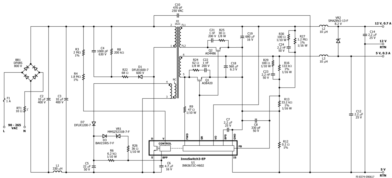
Figure 3 – Schematic.
