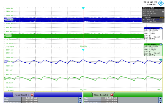
Figure 53 – Output Voltage ripple Waveforms. 265 VAC Input. 5 V PK : 22 mV, 12 V PK : 50 mV. Upper: 5 V, 20 mV / div. Lower: 12 V, 40 mV / , 10 ms, 20 \mu s / div.
